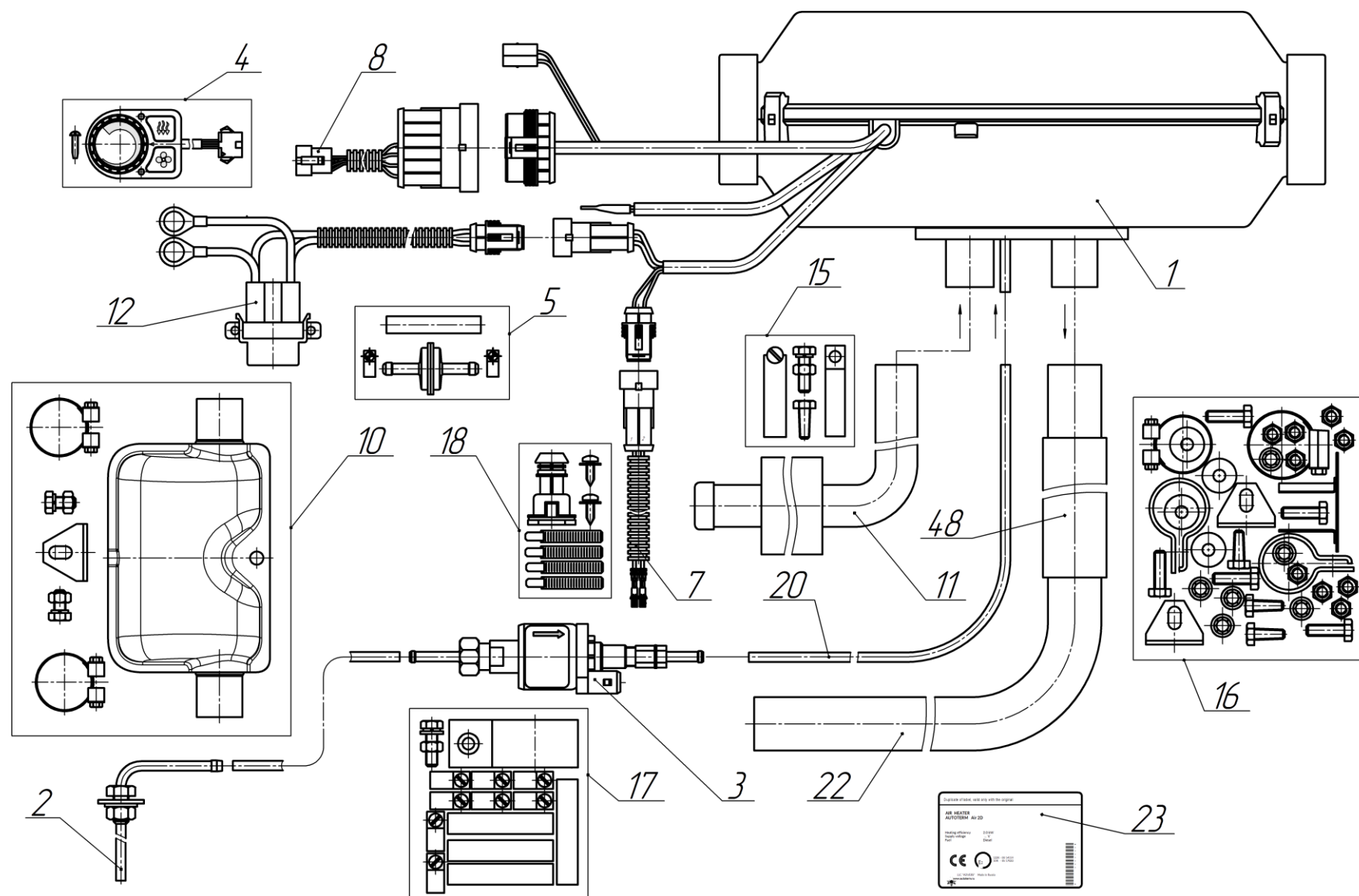
Figure 1 – Contents of the installation kit
